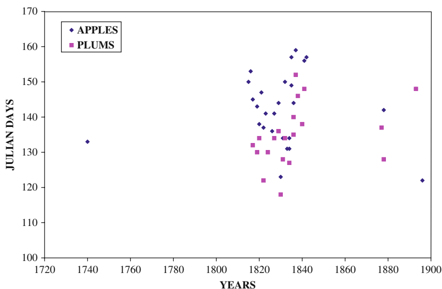
Fig. 3 Full bloom dates for apples and plums observed at Windham, Middlebury and Newbury, VT as well as Concord, Durham and Monroe, NH. Data extracted from the Emory H. Jones, Alexander Miller, Thomas Johnson, Timothy Walker, Nicholas Gilman and Albert Mason diaries respectively. Diary citations are given in the References
