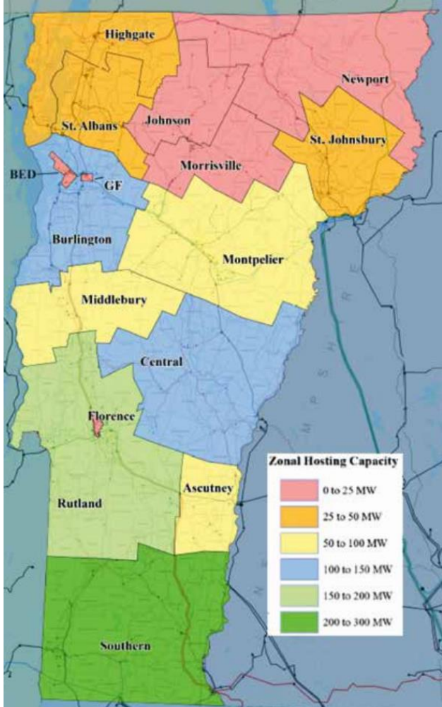
Transmission hosting capacity by region from 2024 VELCO Long-Range Transmission Plan
