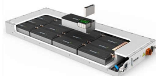
Above: an AKASOL lithium-ion battery for electric buses. Image: greencarcongress.com . Below: cross-section of a battery mounted on the roof of an electric bus. Image: 100percentelectricbuses.wordpress.com .
