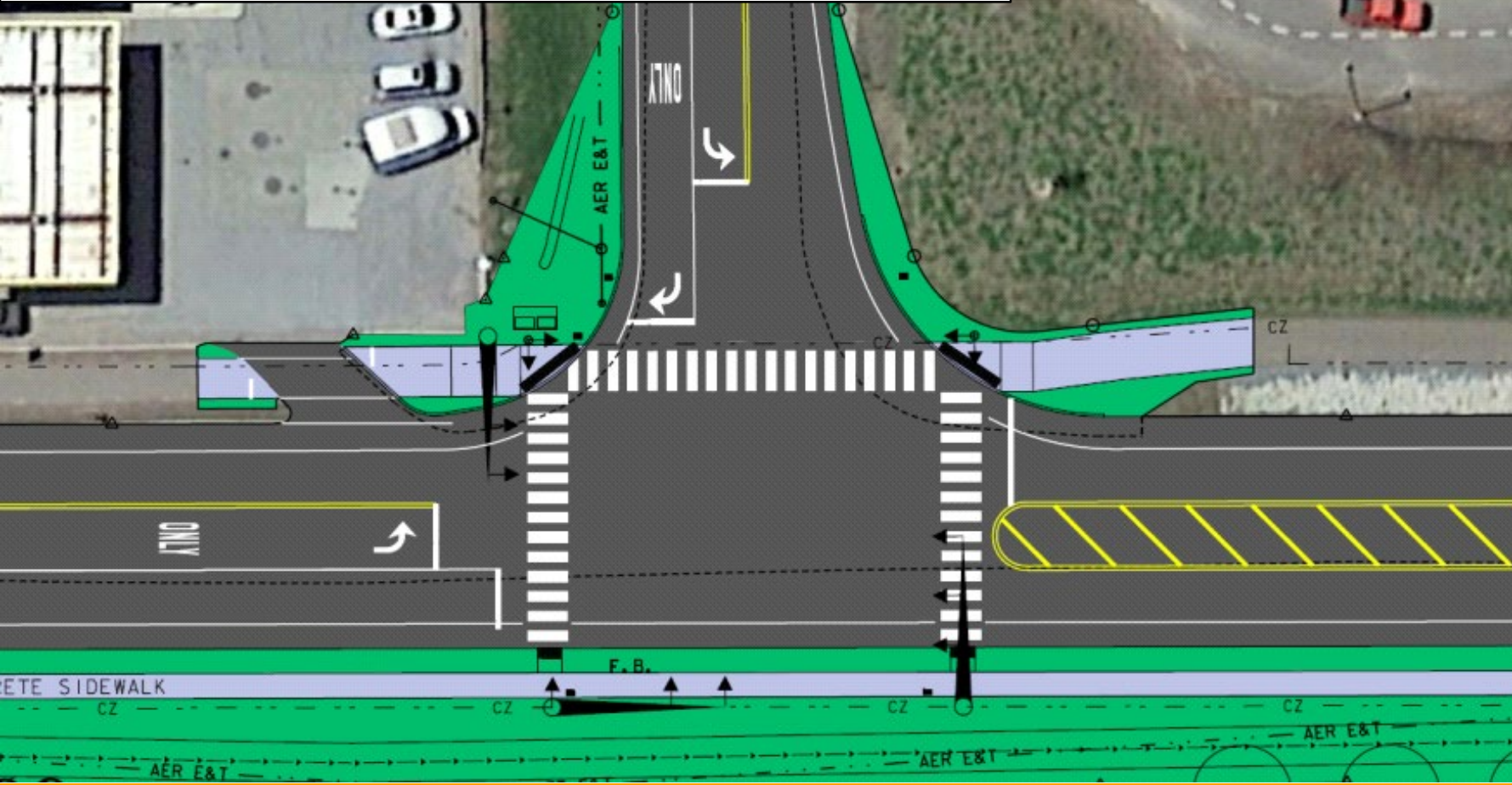
PROPOSED VT ROUTE 2A / JAMES BROWN DRIVE LAYOUT
