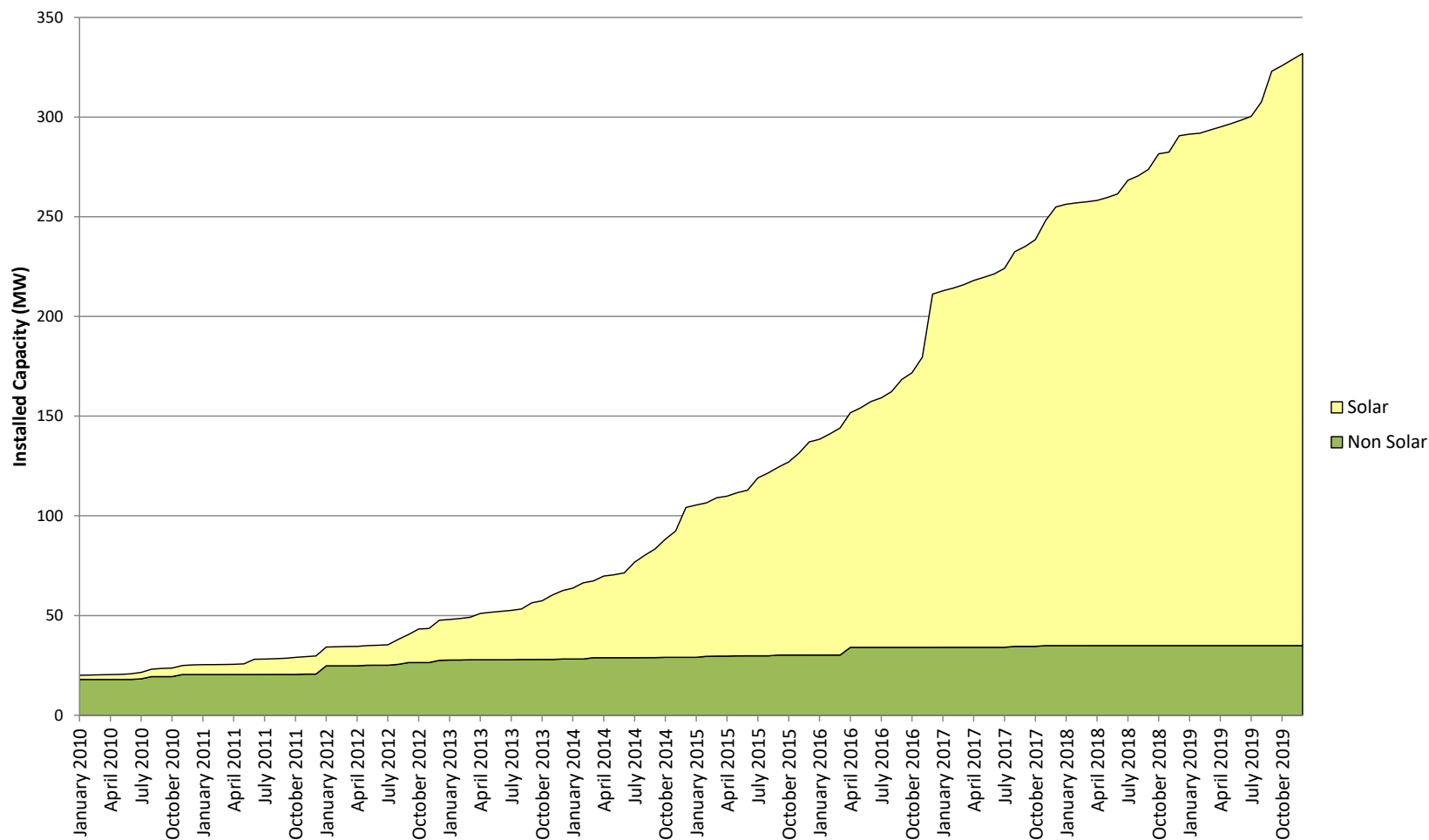
GMP Cumulative Distributed Generation Capacity
