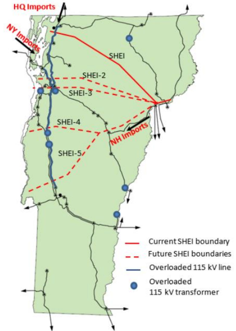
LOCATION OF TRANSMISSION CONSTRAINTS AS A RESULT OF HIGH SOLAR PV
