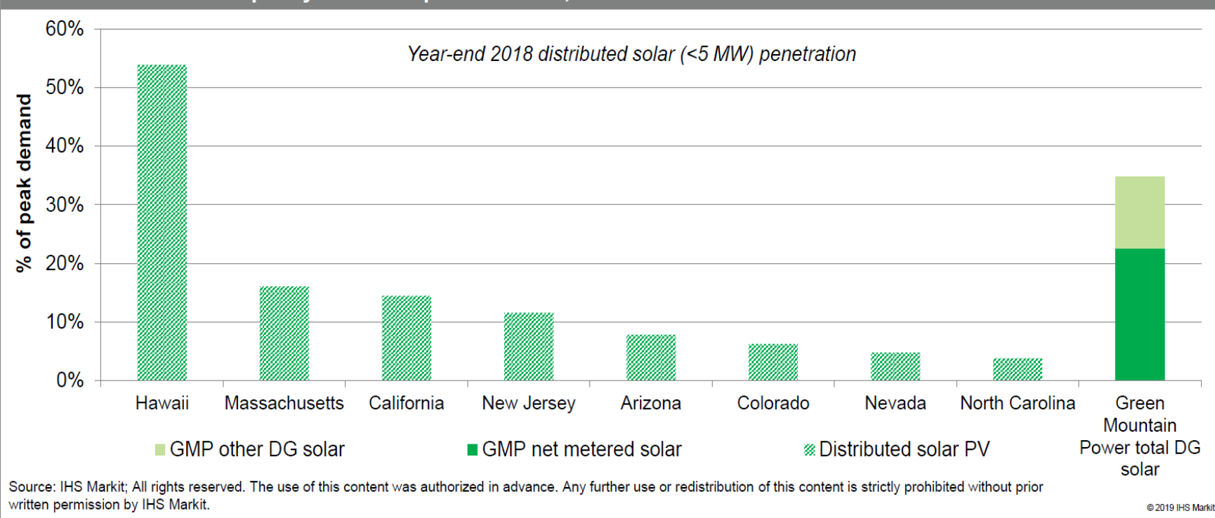
Distributed solar PV capacity as a % of peak demand, 2018
