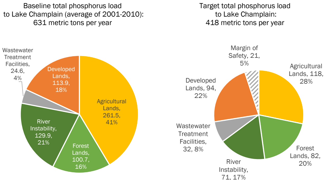
Figure 37. Lake Champlain TMDL baseline (left) and target (right) total phosphorus load in metric tons per year (requires a total reduction of 212.4 metric tons per year) 12
