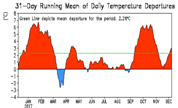
Figure 2. Cooler than normal temperatures in late August allowed Lake Carmi to mix, and then an extended warm spell exacerbated cyanobacteria growth.
