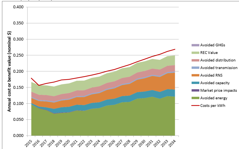
Exhibit 15. Per-kWh costs (red line) and benefits (colored areas) for a 4 kW wing generator installed in 2015, from a ratepayer perspective.
