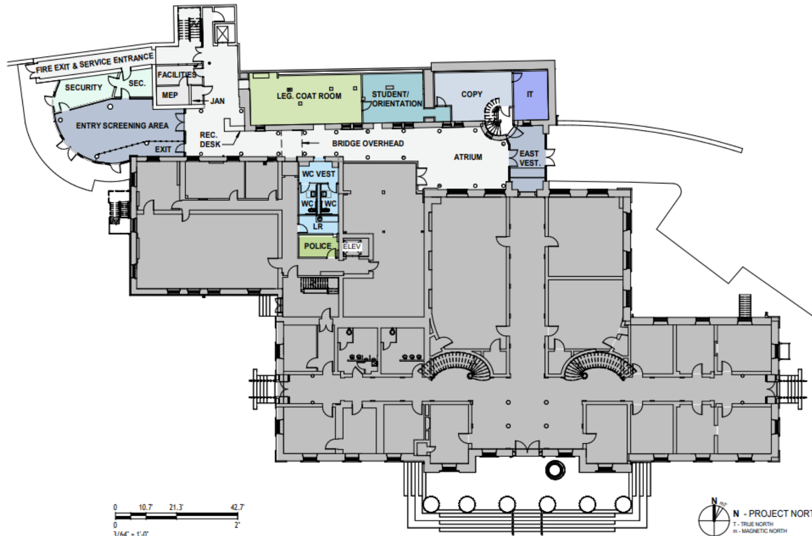
FIRST FLOOR PLAN - OPTION B
