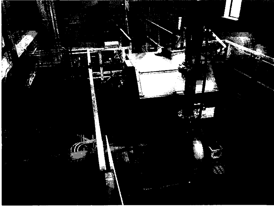
Figure 9: Magnetic drum separator (removes magnetite from CoMag® treated wastewater).
