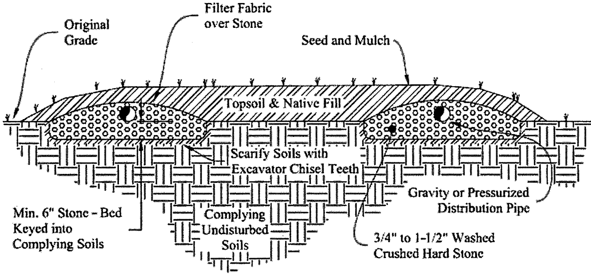
Cross-Section View
