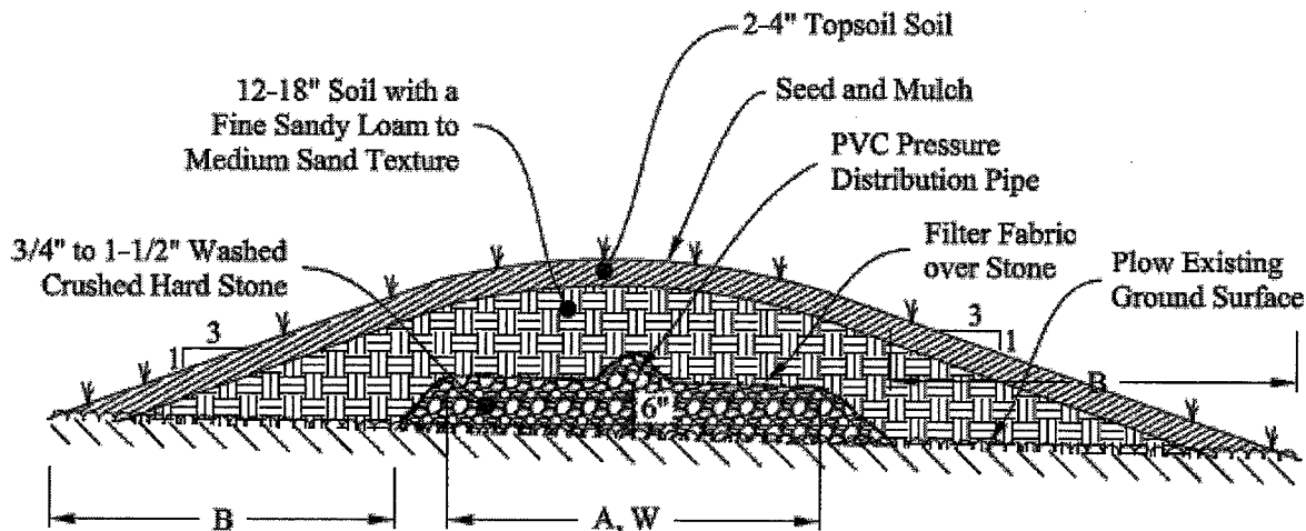
Cross-Section View
