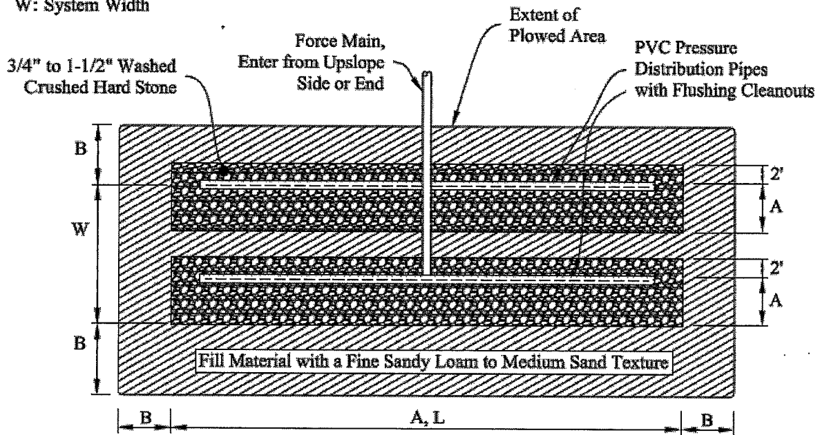
Plan View
