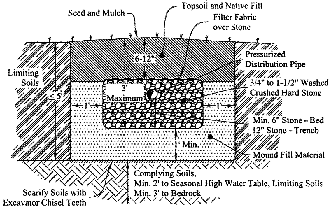
Cross-Section View
