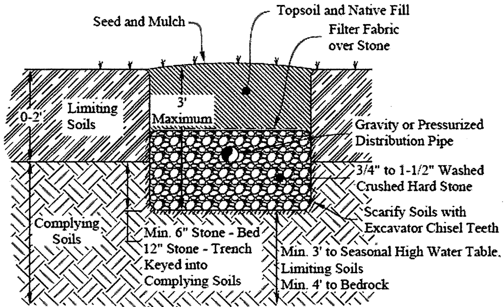
Cross-Section View
