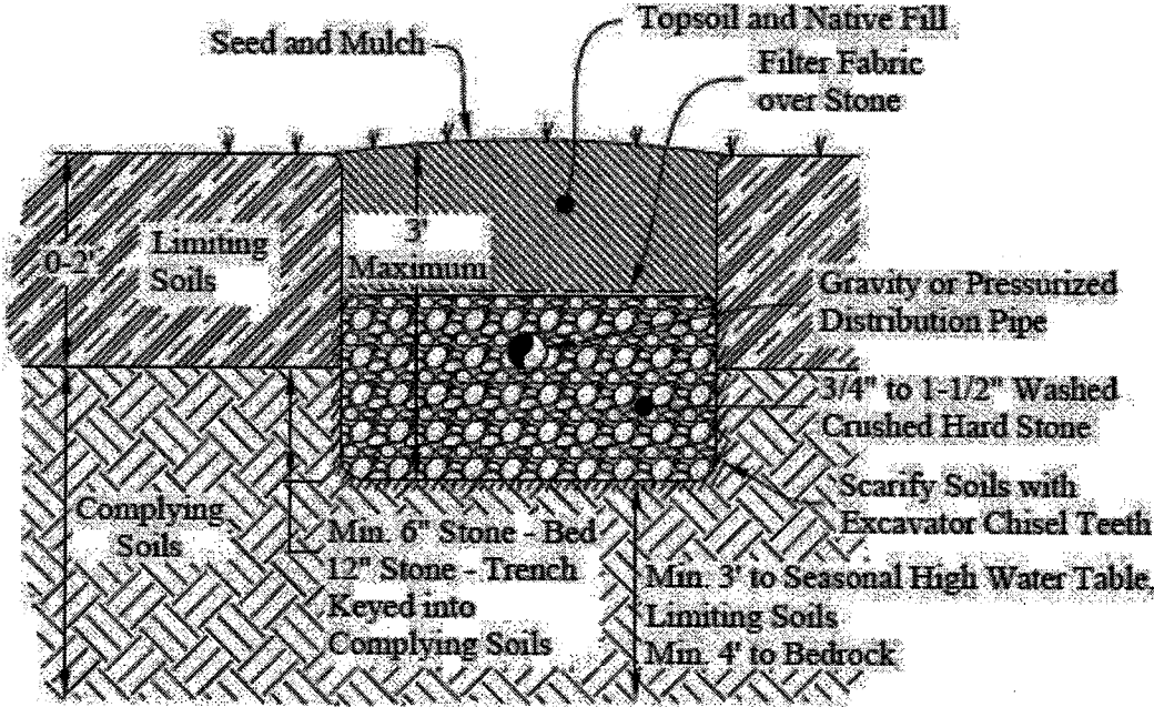
Cross-Section View
