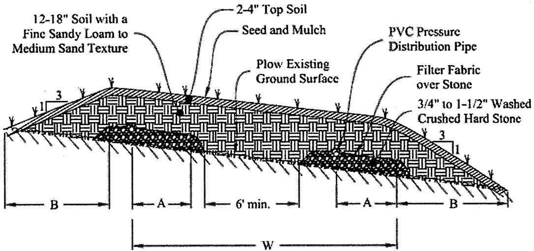
Cross-Section View
