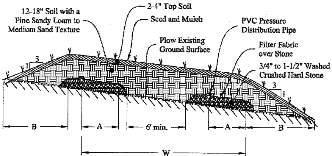
Cross-Section View
